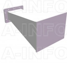
LB-430-10-ASPO Standard Gain Horn Antenna 1.7-2.6GHz 10dB Gain Rectangular Waveguide Interface
